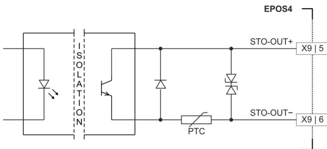
Figure 3-37 STO-OUT circuit
