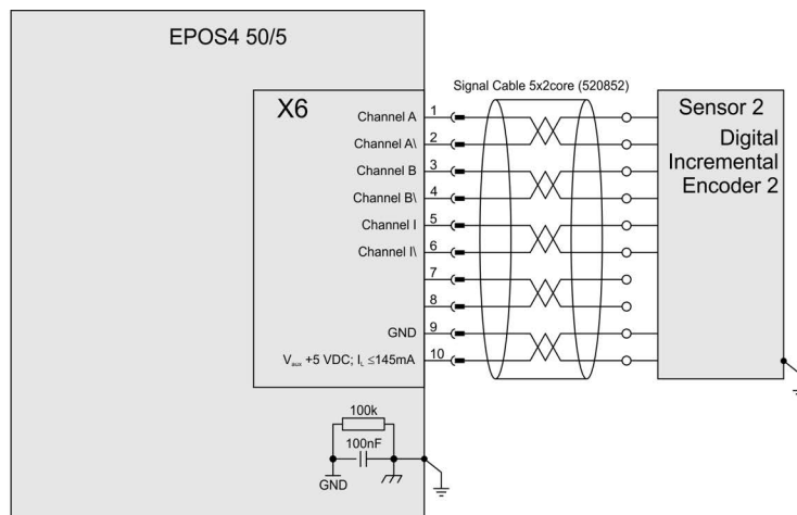
Figure 4-54 Digital incremental encoder 2 (Sensor 2)
