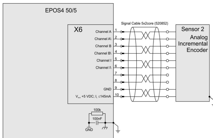
Figure 4-55 Analog incremental encoder (Sensor 2)
