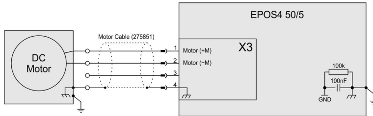
Figure 4-50 DC motor
